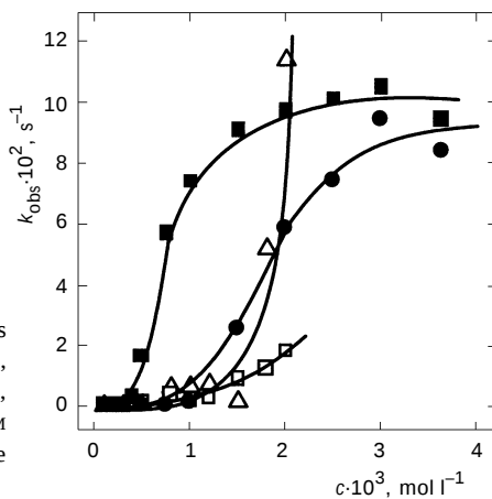
FIG. 1 Rate constant k_{\text{obs}} of the PNPDPP hydrolysis versus surfactant concentration: 2c (□), 2d (●), 2f (■), and 1a (Δ) (ref. 3d ). Conditions: 25 °C, pH 7.2 (0.05 M HEPES buffer and 0.04 M Tris-HBr buffer for ketoximes 2 and aldoxime 1a , respectively)
